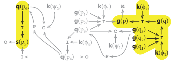
(b) Another consistent (sub)net is highlighted.
