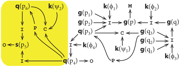
(e) Softgoal approximation is highlighted (Example II.5).
