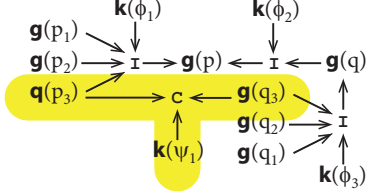
(b) Conflict ( \mathbf{C} ) is highlighted, from Example II.2.
