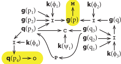
(d) Is-mandatory ( \mathbf{M} ) and is-optional ( \mathbf{O} ) are highlighted, from Example II.4.
