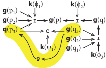
(c) Preference ( \mathbf{P} ) is highlighted, from Example II.3.
